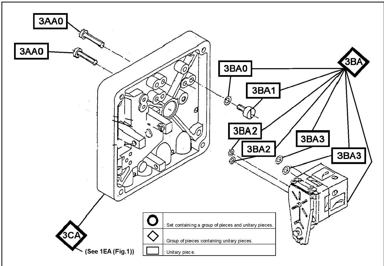
Pneumatic Part (single-acting) (Fig. 3)
